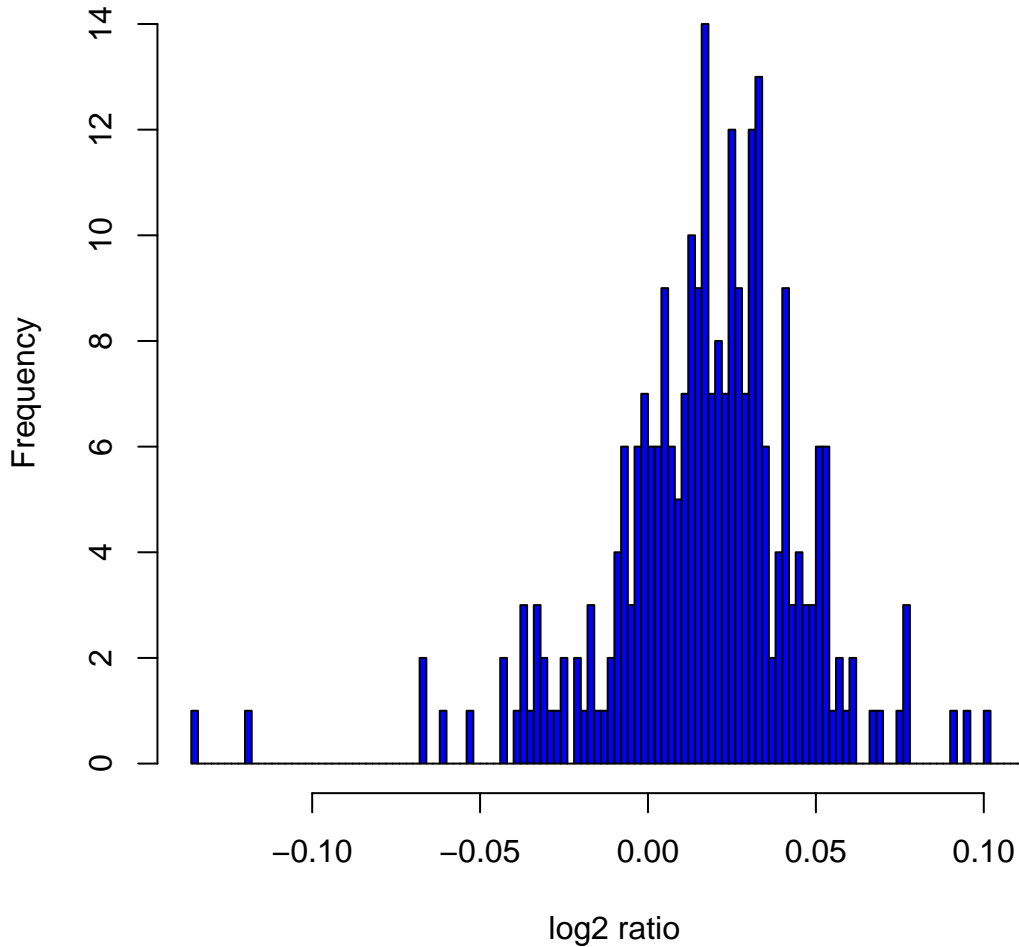
Histogram of log 2 ratios in 270 HapMap samples at clone Chr10tp-9G8
