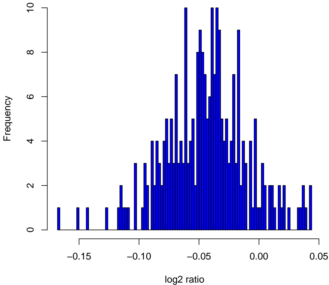
Histogram of log 2 ratios in 270 HapMap samples at clone Chr10tp-9H1
