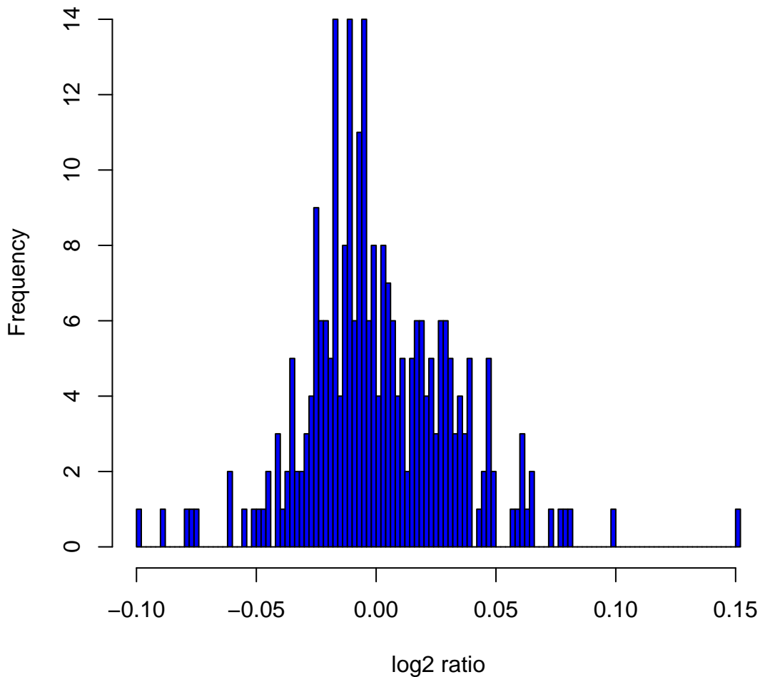
Histogram of log2ratios in 270 HapMap samples at clone Chr10tp-9H12
