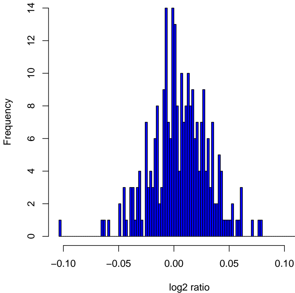
Histogram of log2ratios in 270 HapMap samples at clone Chr11tp-11C2
