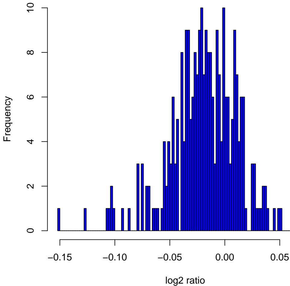
Histogram of log2ratios in 270 HapMap samples at clone Chr11tp-11D4
