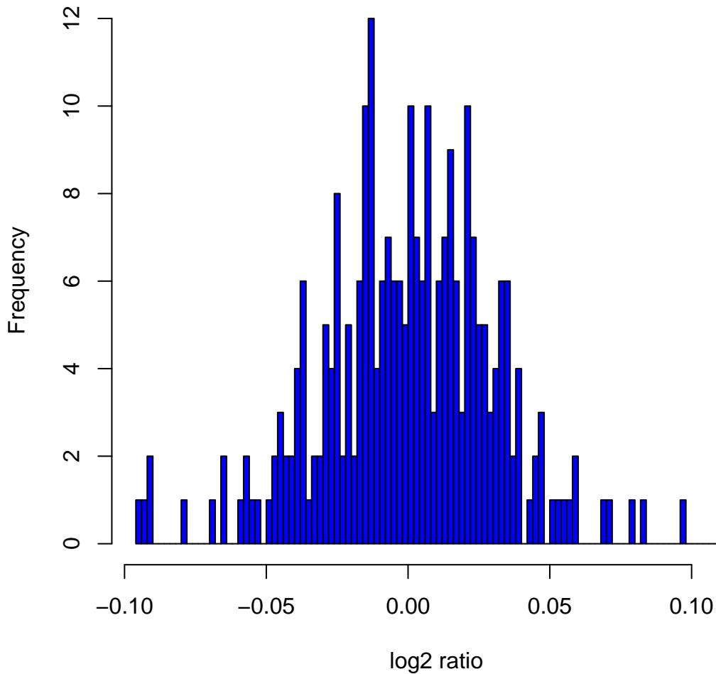
Histogram of log2ratios in 270 HapMap samples at clone Chr11tp-12A7
