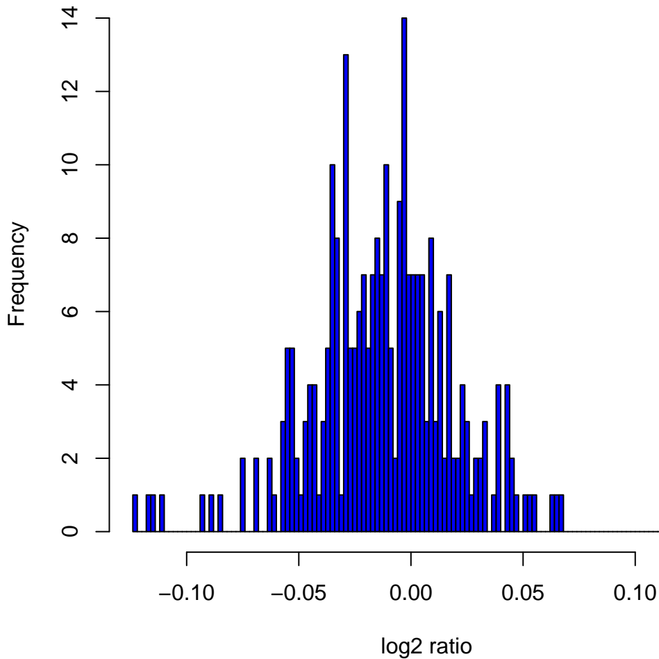
Histogram of log2ratios in 270 HapMap samples at clone Chr11tp-13A3
