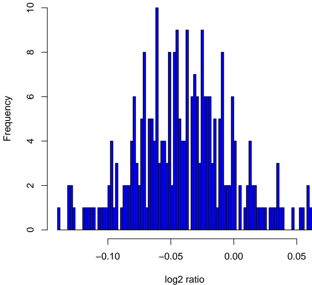
Histogram of log2ratios in 270 HapMap samples at clone Chr11tp-13A8
