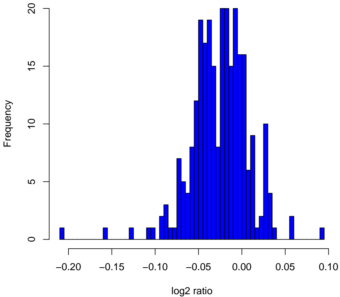
Histogram of log2ratios in 270 HapMap samples at clone Chr11tp-13B10
