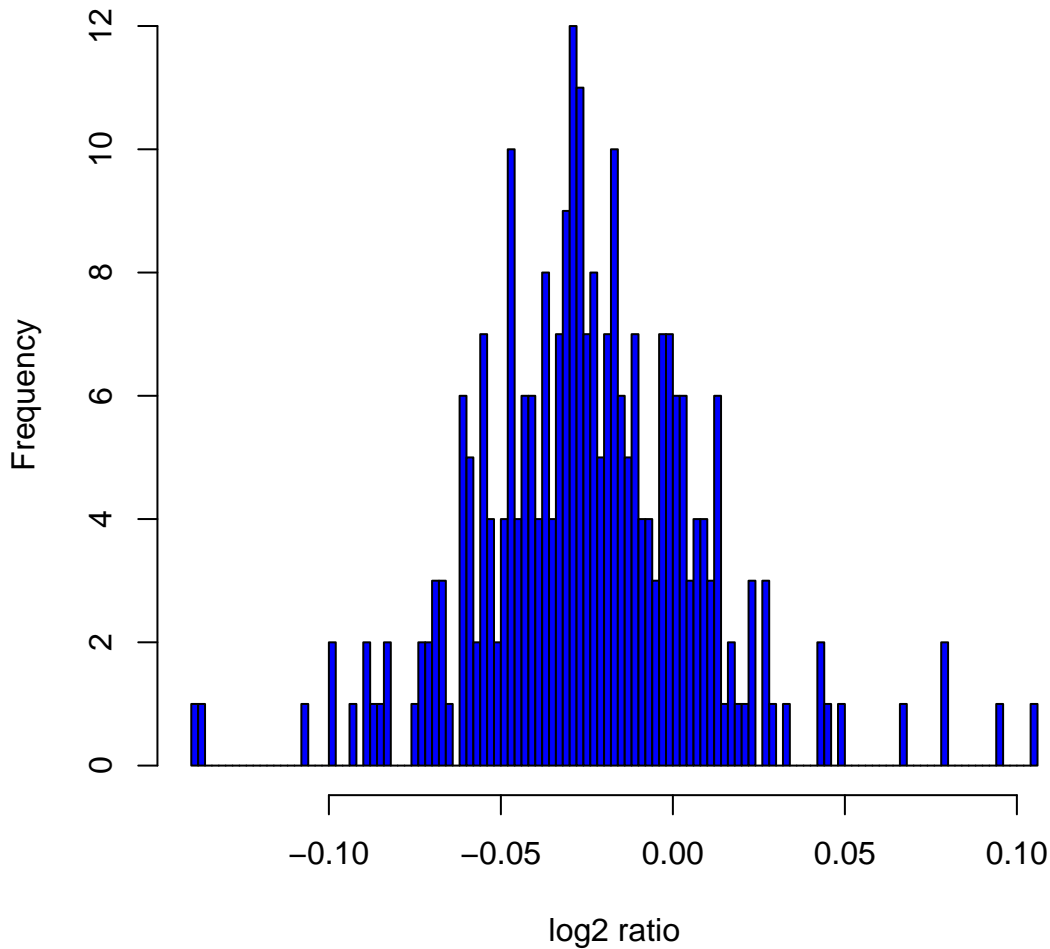
Histogram of log2ratios in 270 HapMap samples at clone Chr11tp-13B5
