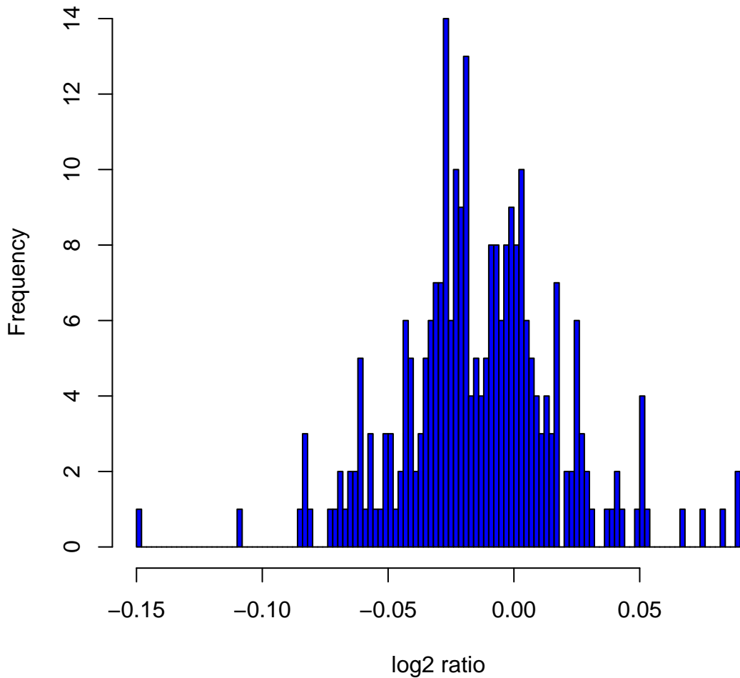
Histogram of log2ratios in 270 HapMap samples at clone Chr11tp-13C7
