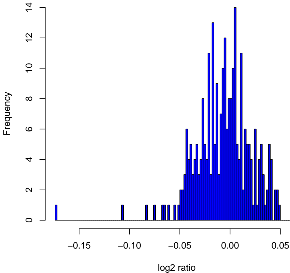
Histogram of log2ratios in 270 HapMap samples at clone Chr11tp-13C8
