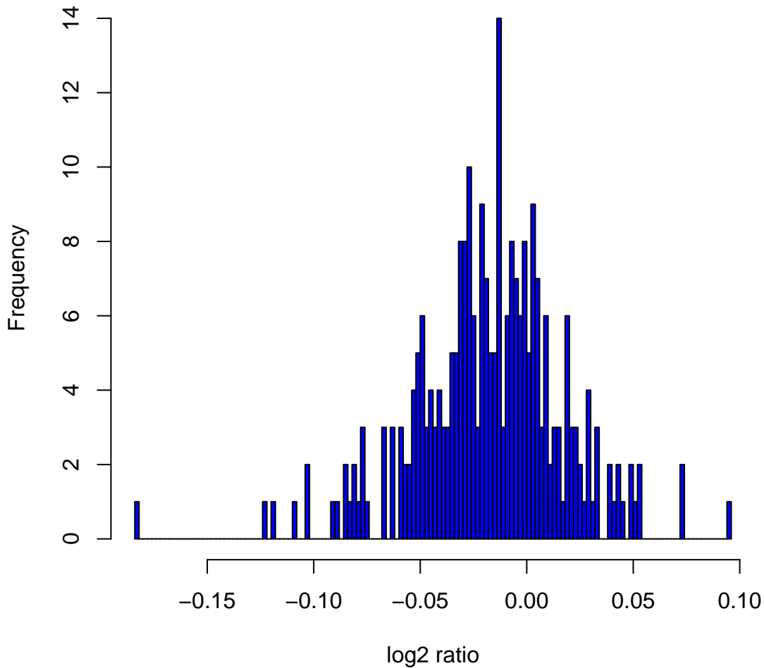
Histogram of log2ratios in 270 HapMap samples at clone Chr11tp-13H3
