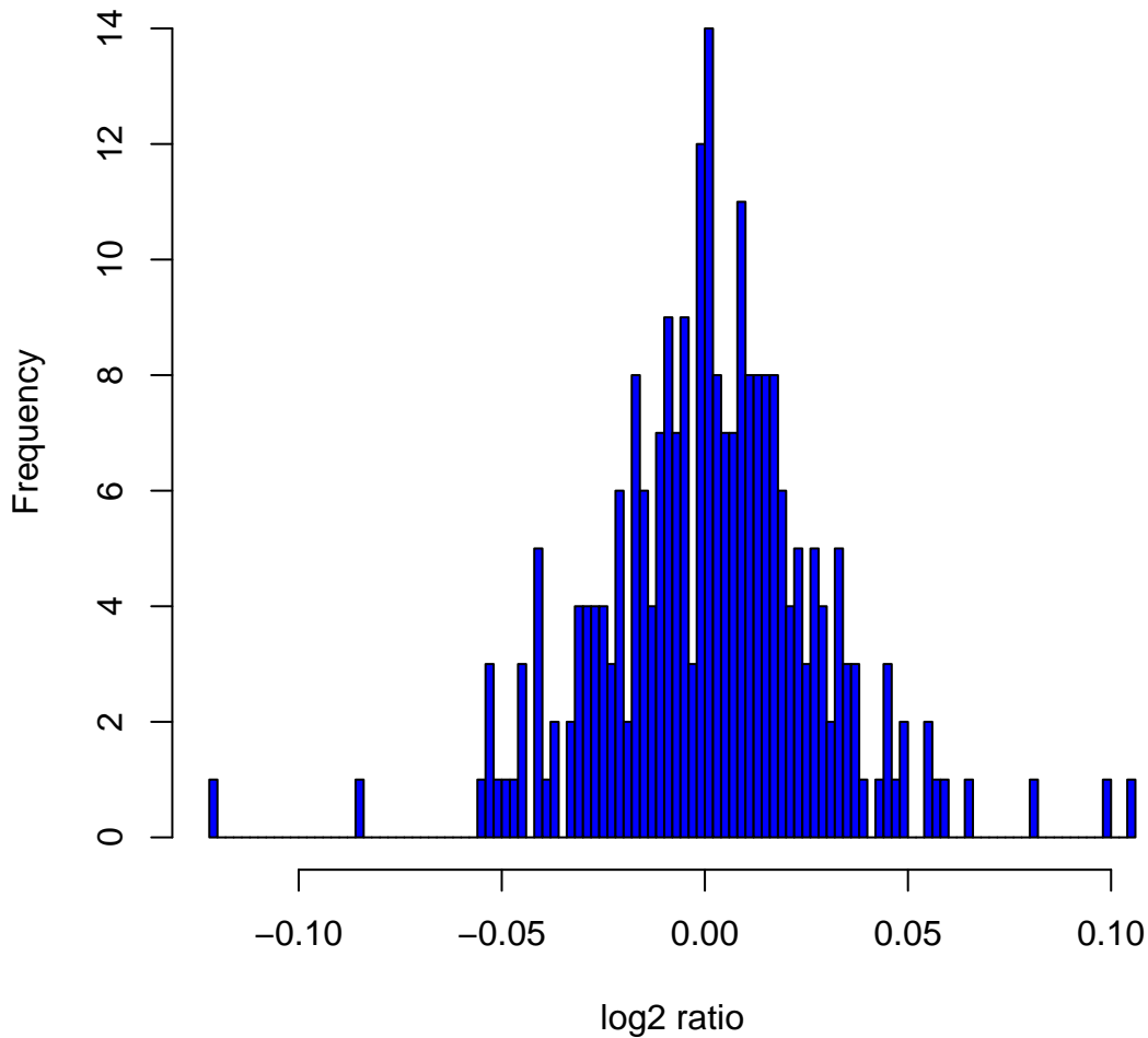
Histogram of log2ratios in 270 HapMap samples at clone Chr11tp-13H6
