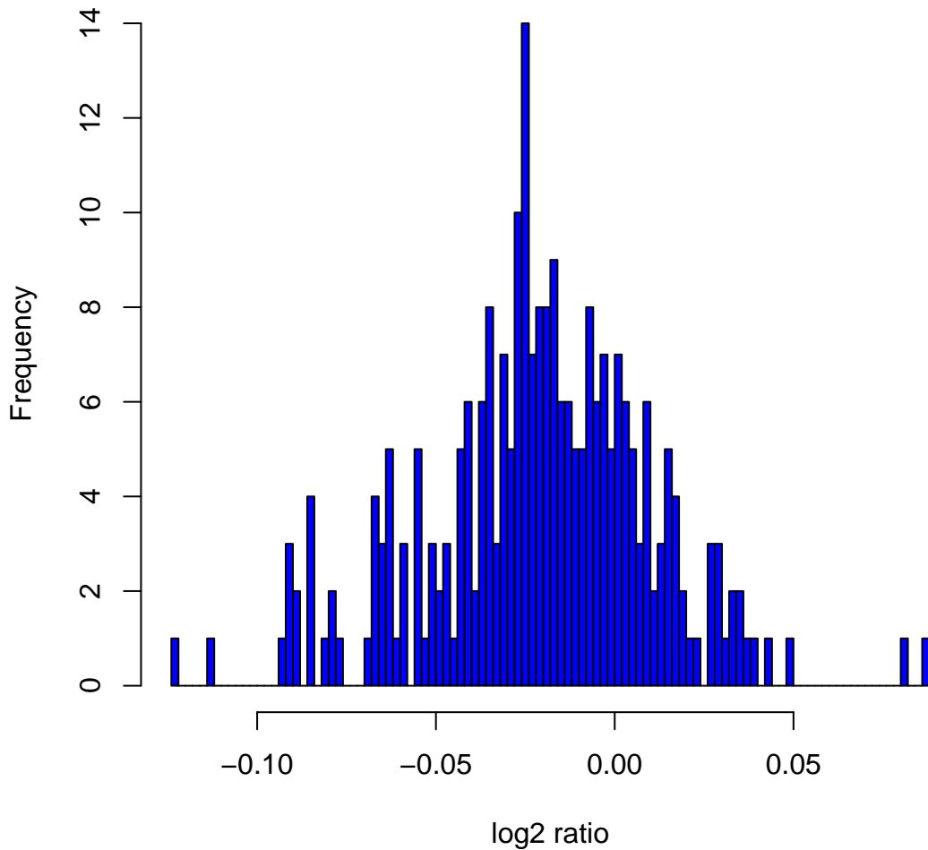
Histogram of log2ratios in 270 HapMap samples at clone Chr11tp-13H8
