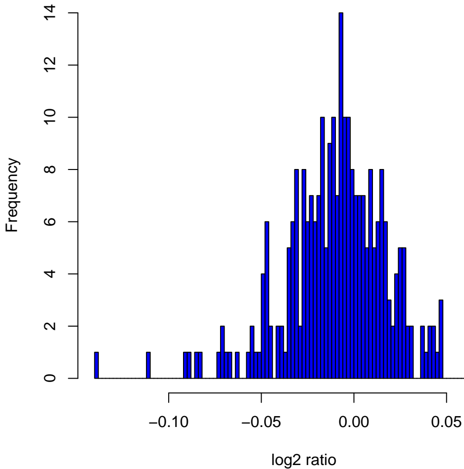
Histogram of log2ratios in 270 HapMap samples at clone Chr11tp-14D9
