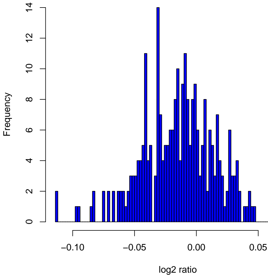
Histogram of log2ratios in 270 HapMap samples at clone Chr11tp-14G8
