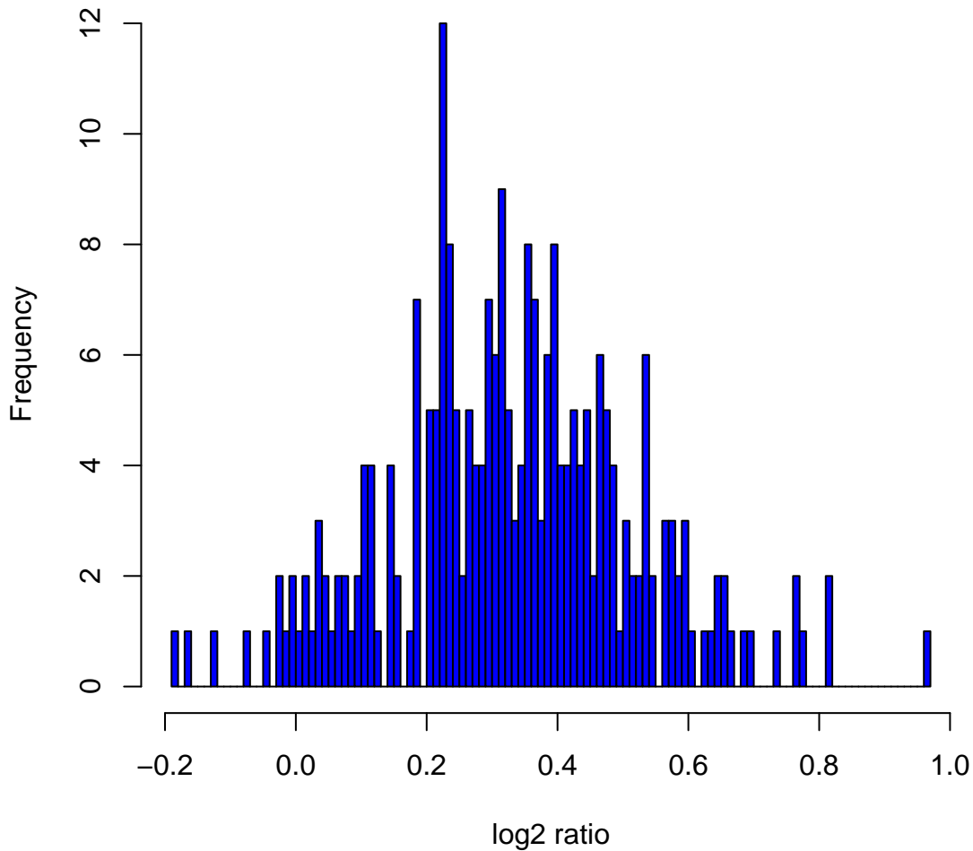
Histogram of log2ratios in 270 HapMap samples at clone Chr11tp-14H12
