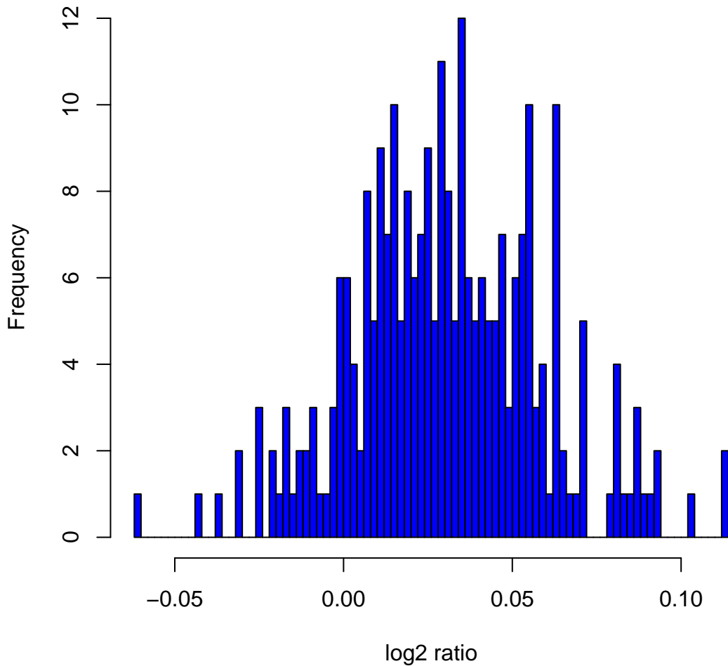
Histogram of log2ratios in 270 HapMap samples at clone Chr11tp-14H3
