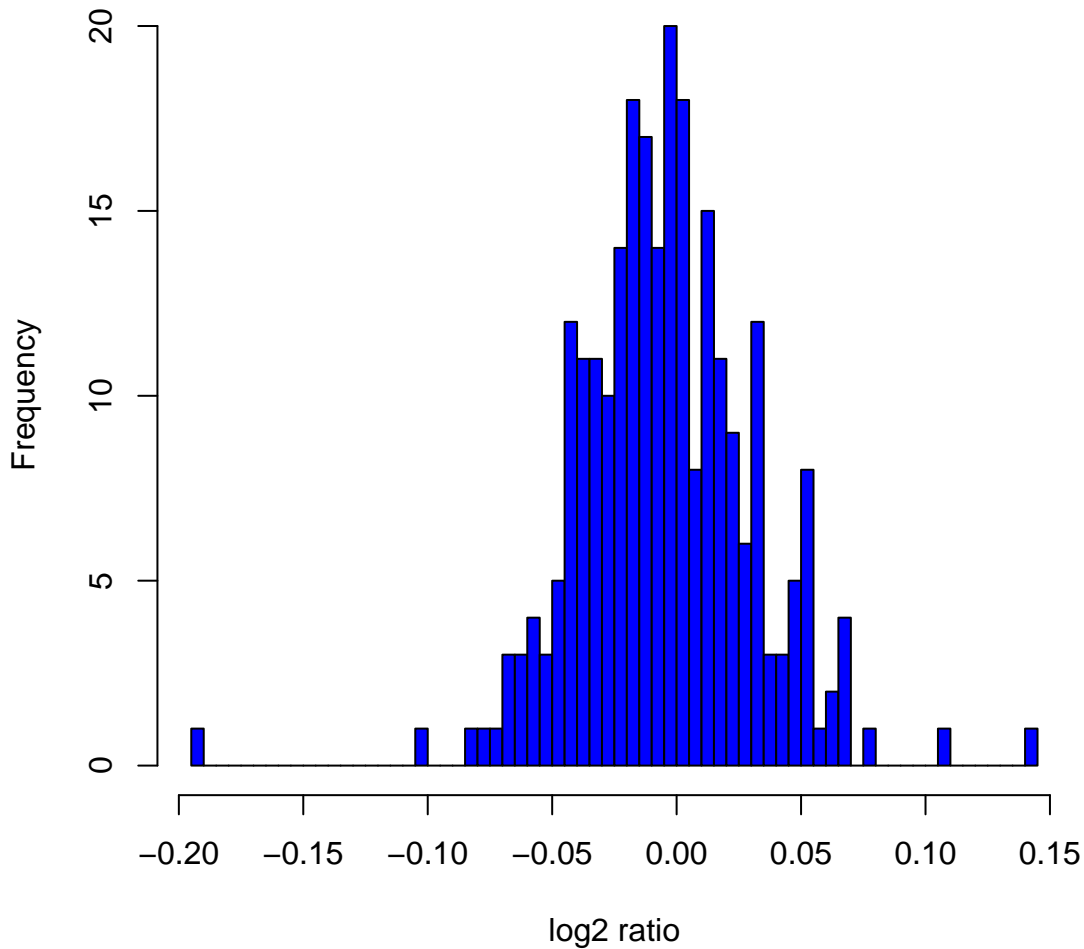
Histogram of log2ratios in 270 HapMap samples at clone Chr11tp-15D9
