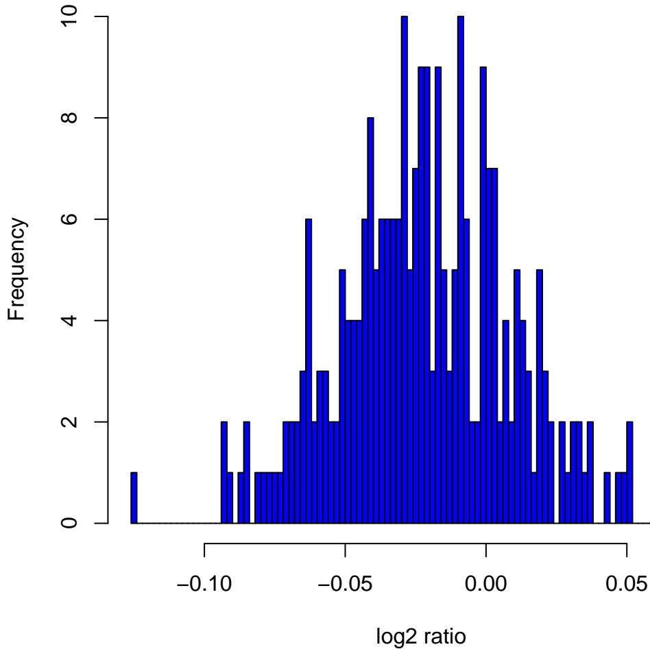
Histogram of log2ratios in 270 HapMap samples at clone Chr11tp-15F7
