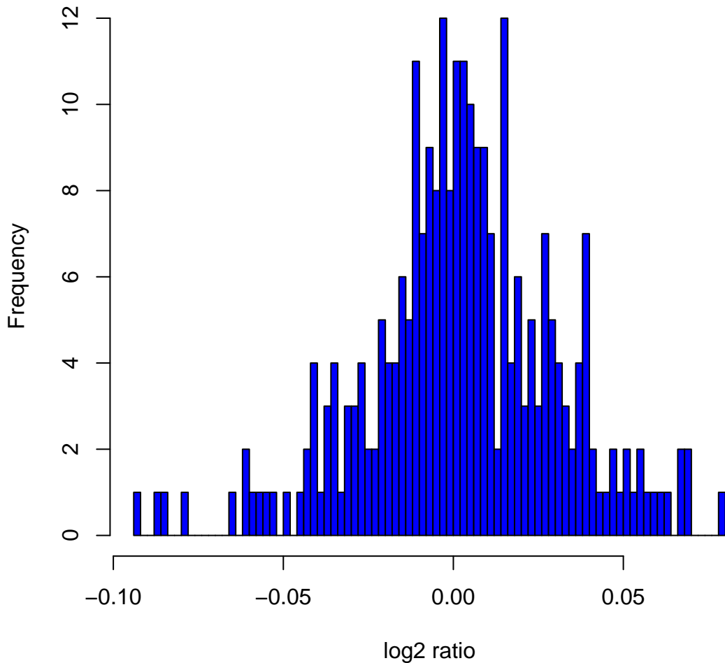
Histogram of log2ratios in 270 HapMap samples at clone Chr11tp-15G10
