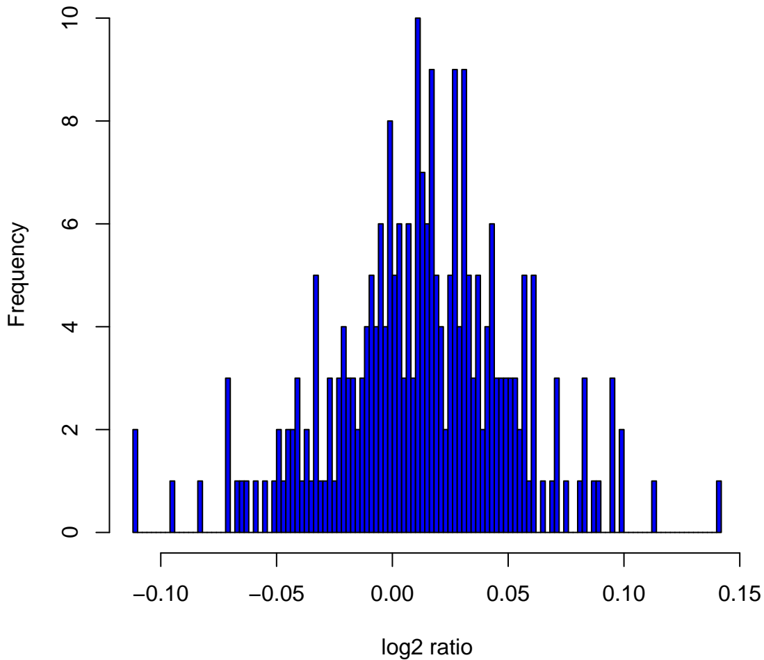
Histogram of log2ratios in 270 HapMap samples at clone Chr11tp-16D8
