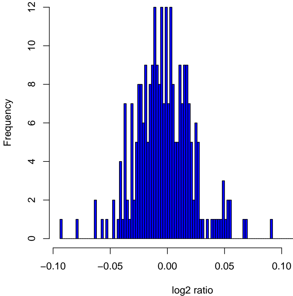
Histogram of log2ratios in 270 HapMap samples at clone Chr11tp-17A1
