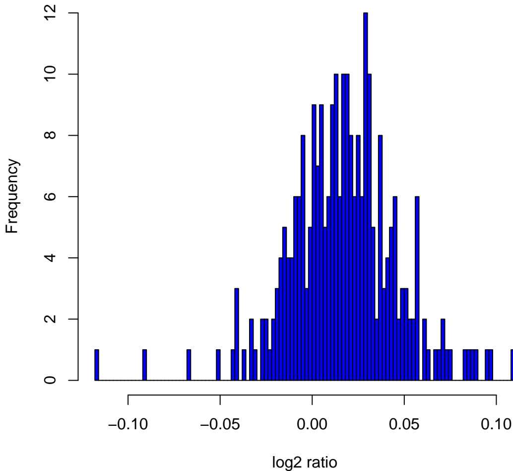
Histogram of log2ratios in 270 HapMap samples at clone Chr11tp-17B3
