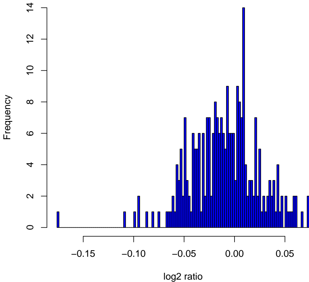
Histogram of log2ratios in 270 HapMap samples at clone Chr11tp-17B9
