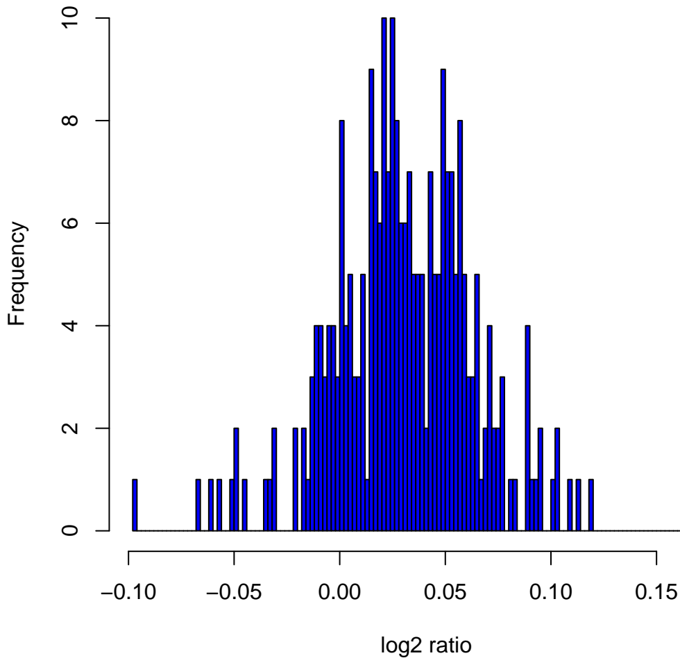
Histogram of log2ratios in 270 HapMap samples at clone Chr11tp-17D7
