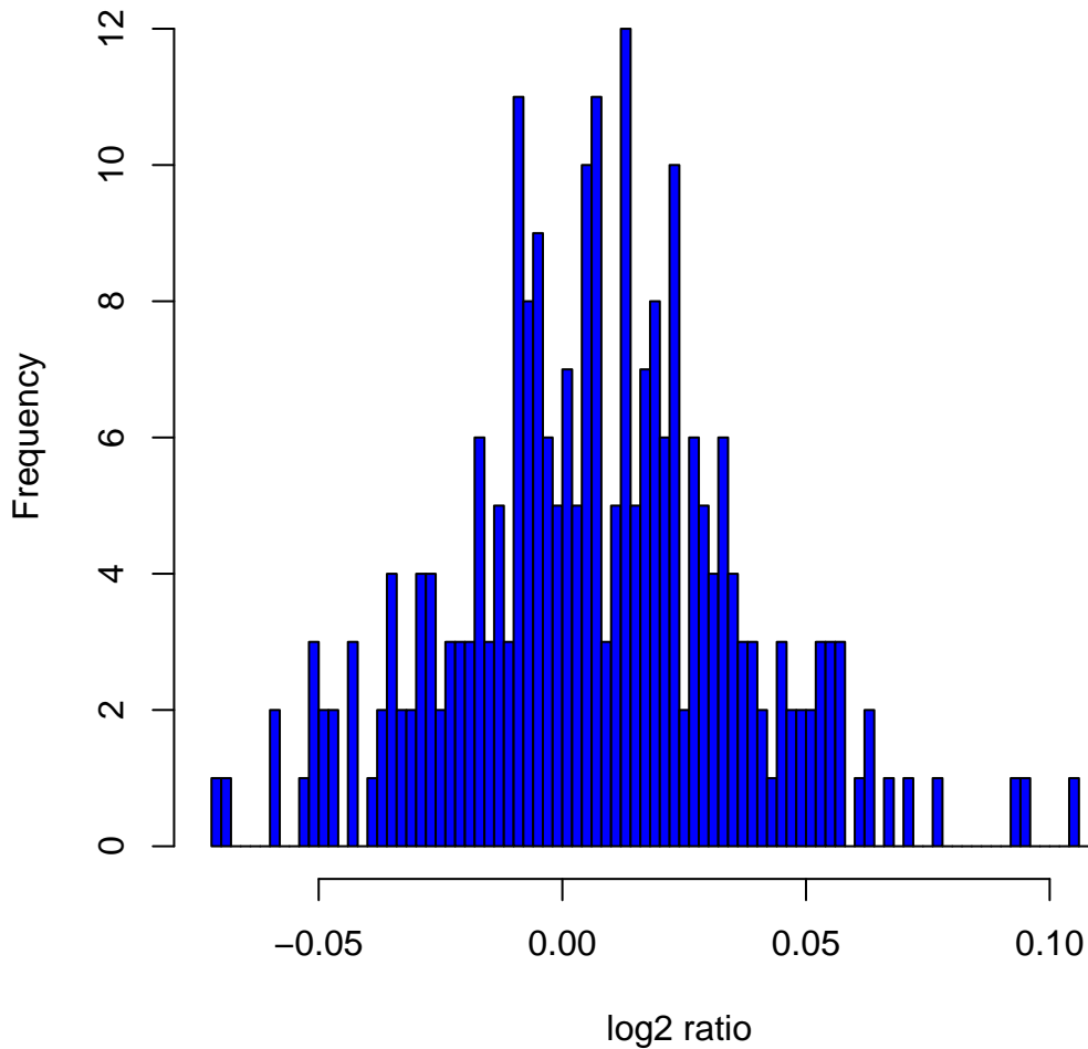
Histogram of log2ratios in 270 HapMap samples at clone Chr11tp-17D9
