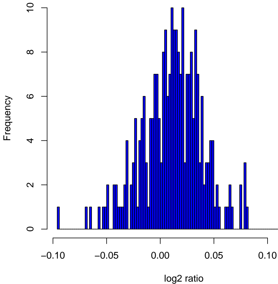
Histogram of \log_2 ratios in 270 HapMap samples at clone Chr11tp-17G3
