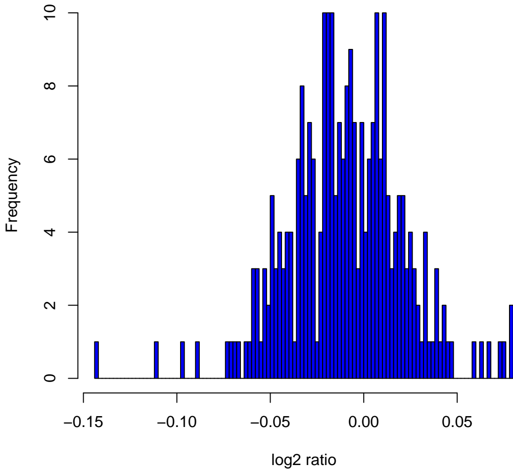
Histogram of log2ratios in 270 HapMap samples at clone Chr11tp-18A4
