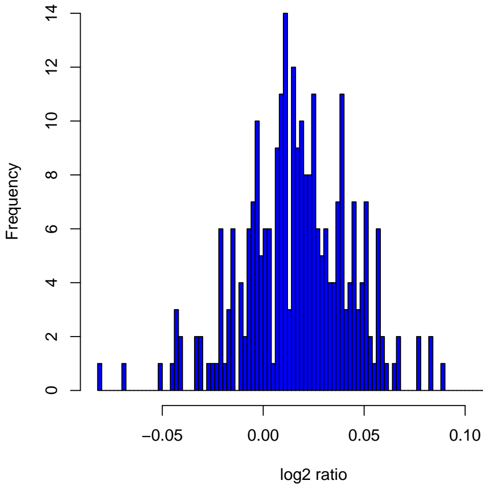
Histogram of log2ratios in 270 HapMap samples at clone Chr11tp-18A7
