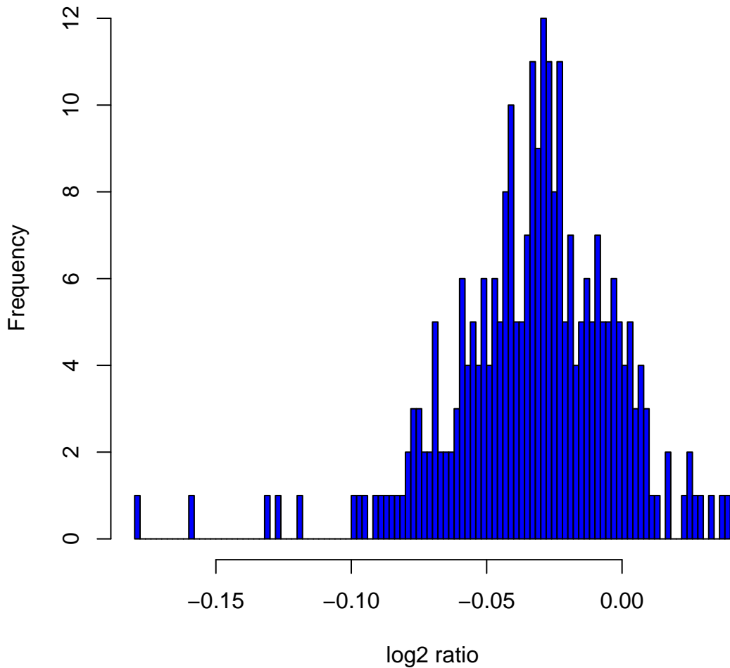
Histogram of log2ratios in 270 HapMap samples at clone Chr11tp-18B7
