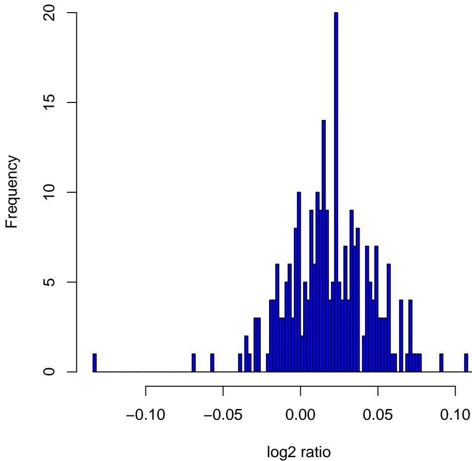
Histogram of log2ratios in 270 HapMap samples at clone Chr11tp-18D2
