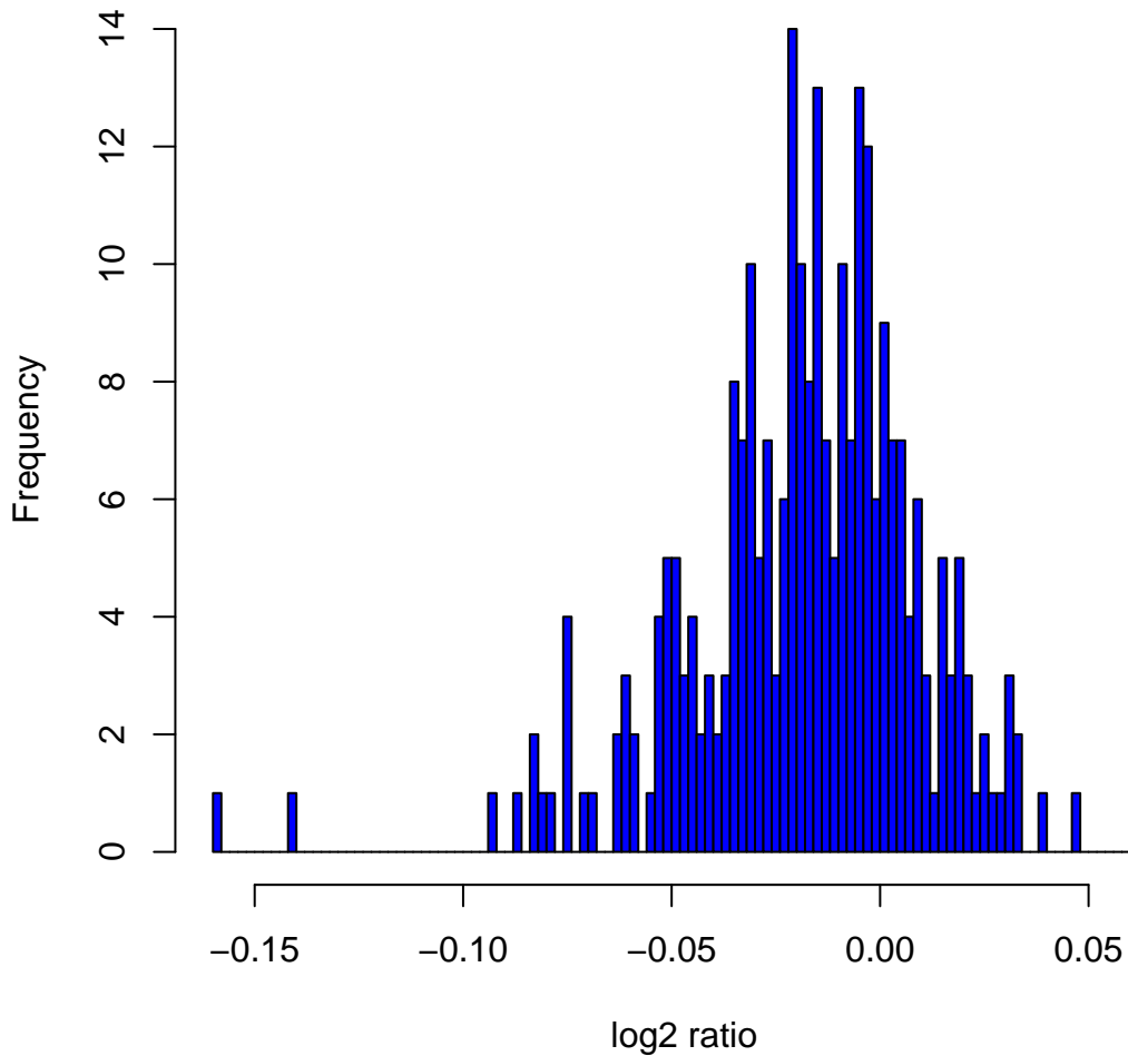
Histogram of log2ratios in 270 HapMap samples at clone Chr11tp-18D7
