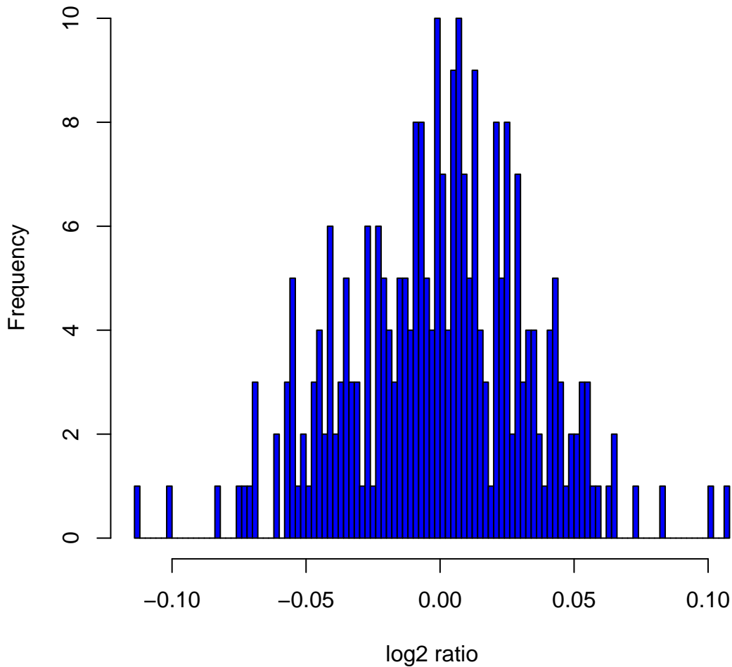
Histogram of log2ratios in 270 HapMap samples at clone Chr11tp-18E2
