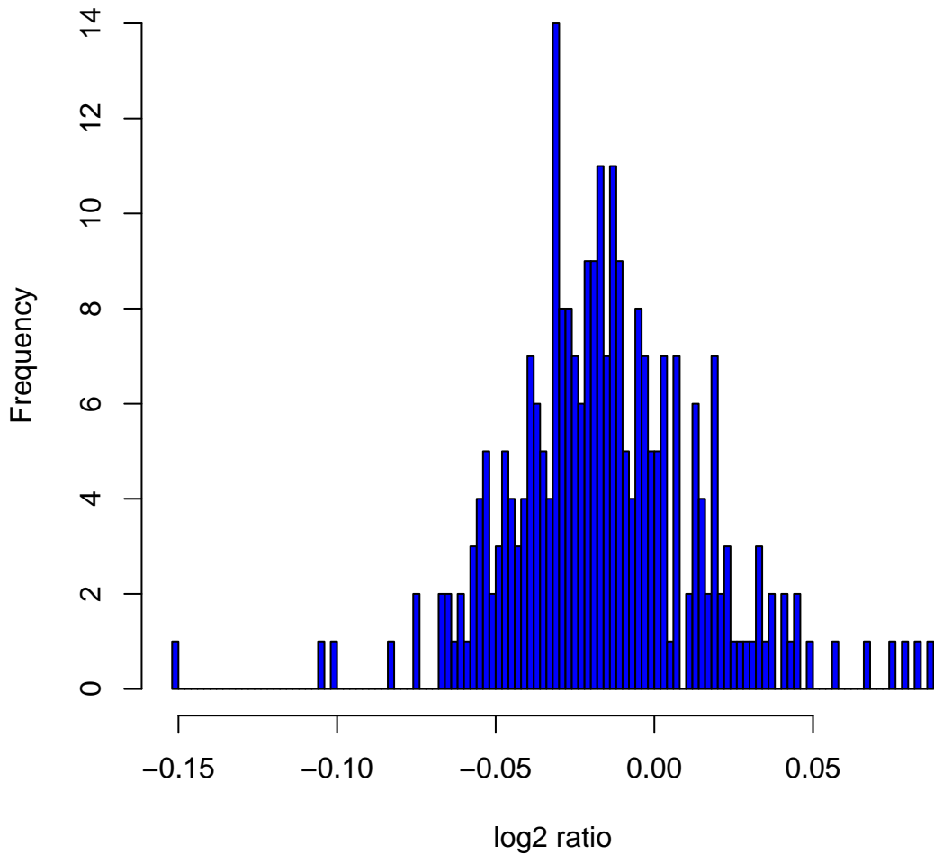
Histogram of log2ratios in 270 HapMap samples at clone Chr11tp-18E7
