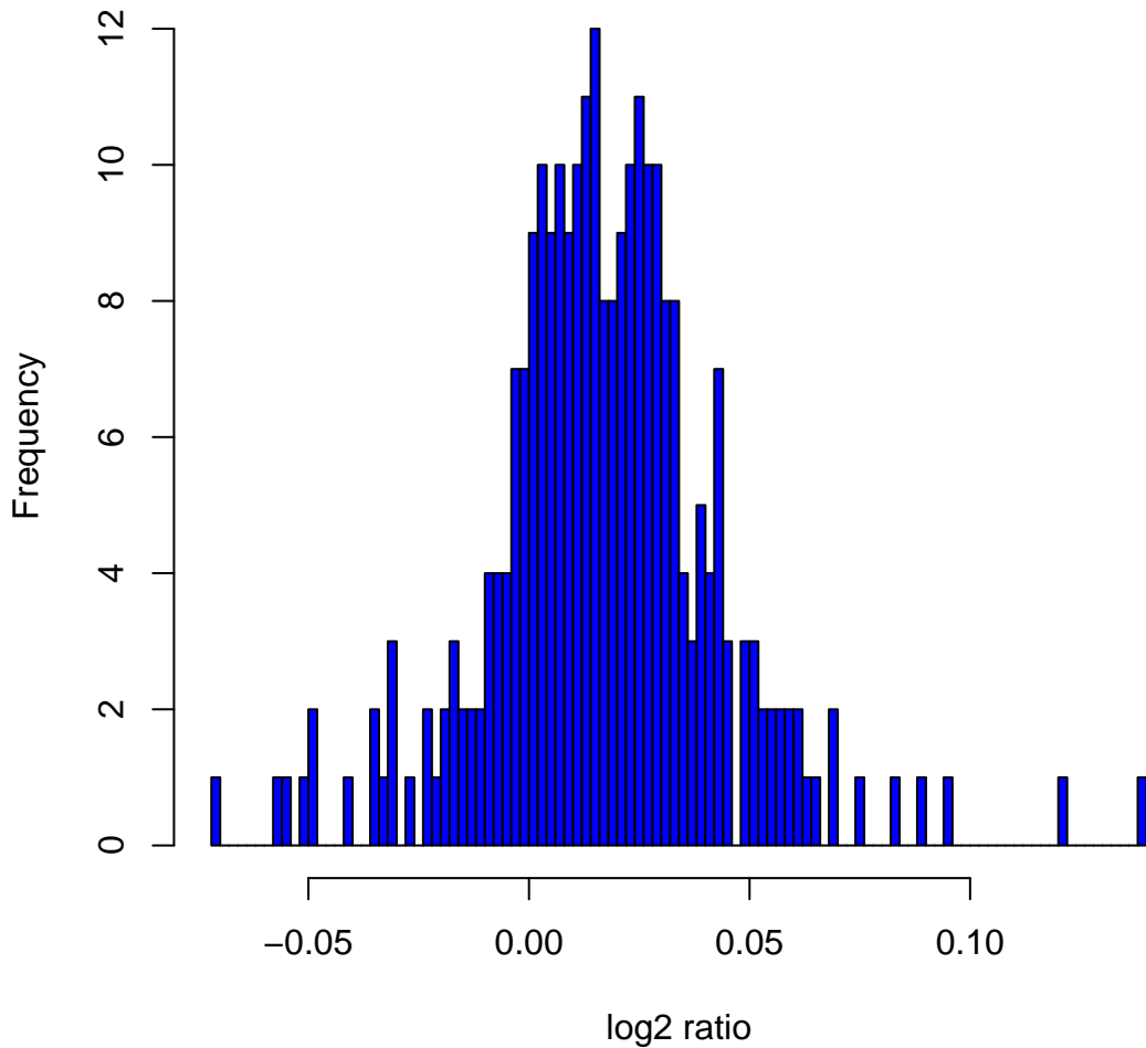
Histogram of log 2 ratios in 270 HapMap samples at clone Chr11tp-1B6
