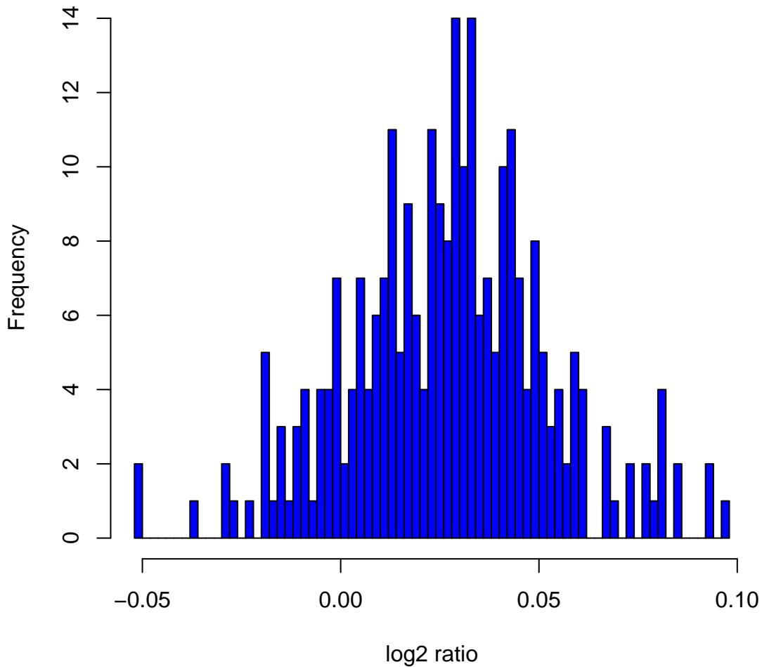
Histogram of log2ratios in 270 HapMap samples at clone Chr11tp-1G1
