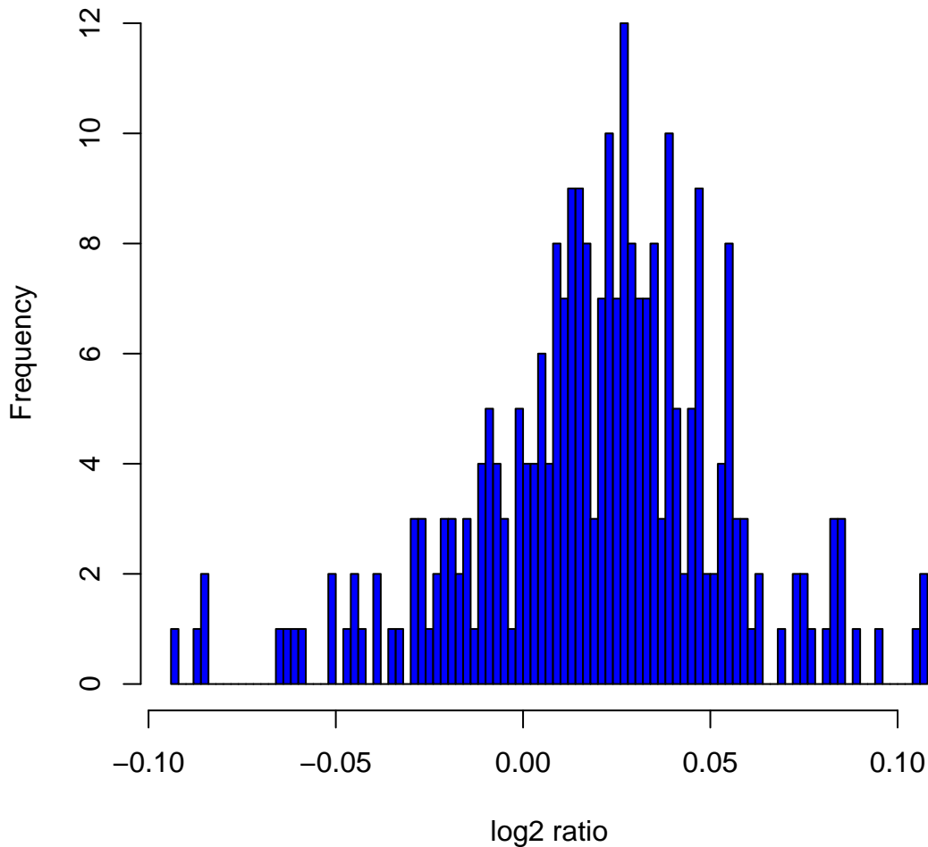
Histogram of log 2 ratios in 270 HapMap samples at clone Chr11tp-1H8
