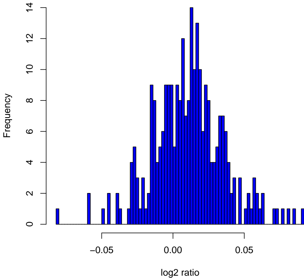
Histogram of log 2 ratios in 270 HapMap samples at clone Chr11tp-2G2
