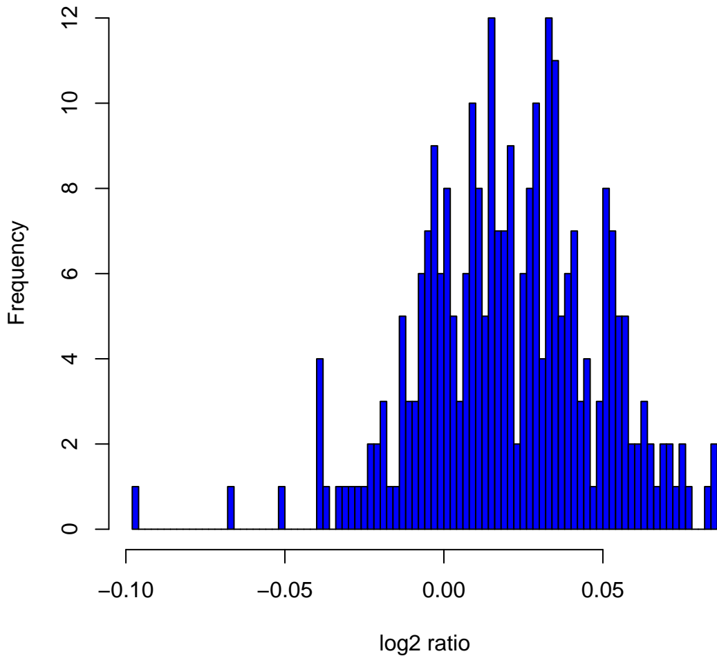
Histogram of log2ratios in 270 HapMap samples at clone Chr11tp-3A10
