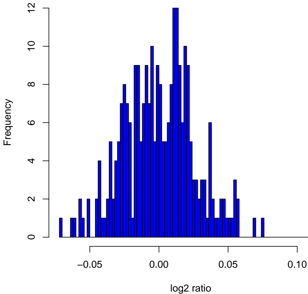
Histogram of log 2 ratios in 270 HapMap samples at clone Chr11tp-3A9
