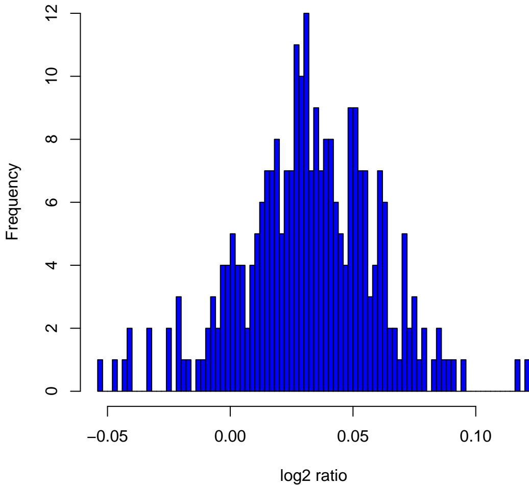
Histogram of log 2 ratios in 270 HapMap samples at clone Chr11tp-3C8
