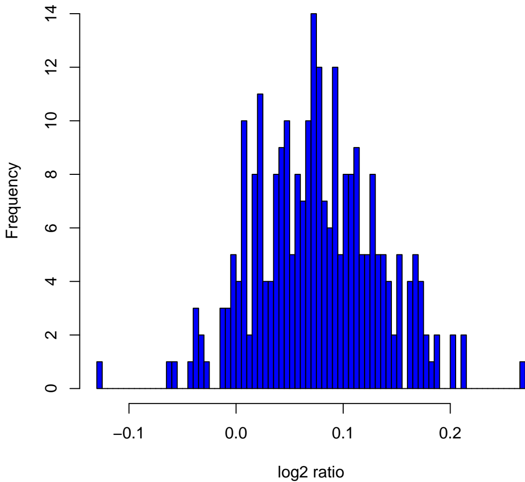
Histogram of log2ratios in 270 HapMap samples at clone Chr11tp-3H7
