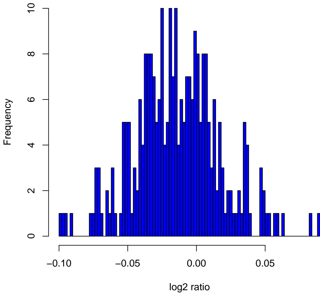
Histogram of log 2 ratios in 270 HapMap samples at clone Chr11tp-3H8
