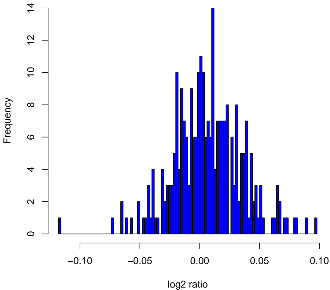
Histogram of log2ratios in 270 HapMap samples at clone Chr11tp-4A10
