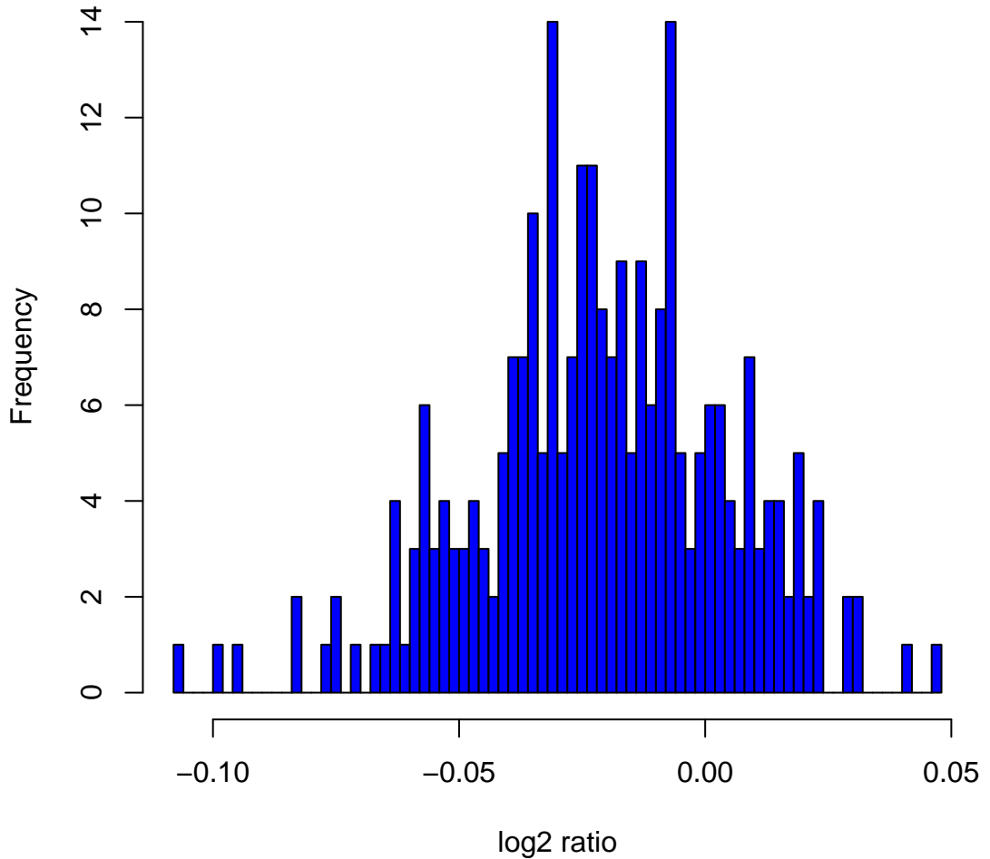
Histogram of log2ratios in 270 HapMap samples at clone Chr11tp-4B11
