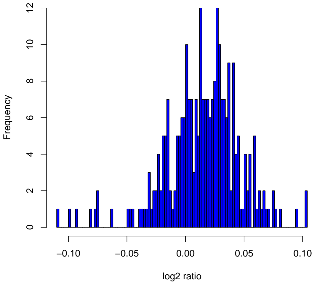
Histogram of log 2 ratios in 270 HapMap samples at clone Chr11tp-4C3
