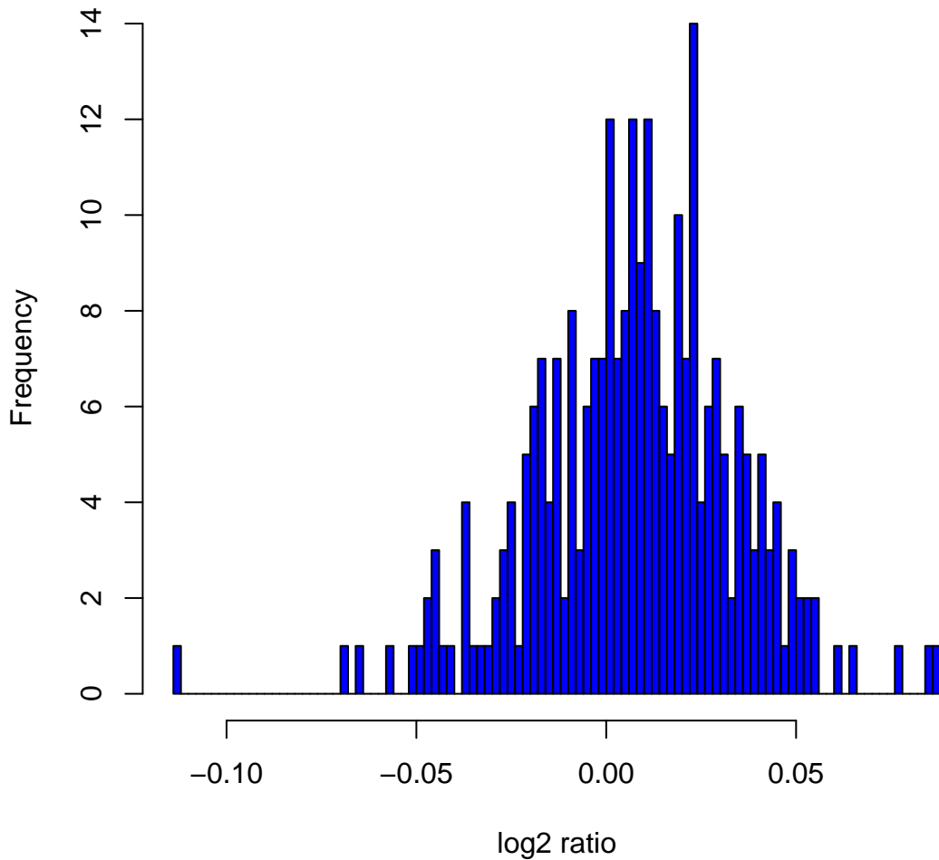
Histogram of log2ratios in 270 HapMap samples at clone Chr11tp-4D10
