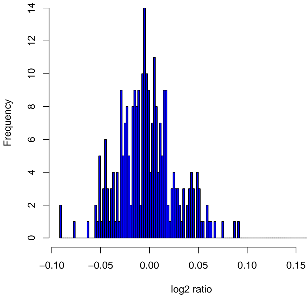
Histogram of \log_2 ratios in 270 HapMap samples at clone Chr11tp-4E8
